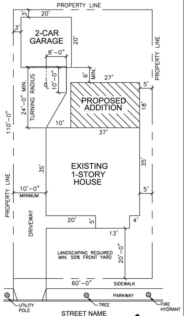
SCALE SHALL NOT BE LESS THAN 1/8" = 1'-0" NORTH PLOT PLAN MUST BE FULLY DIMENSIONED AND TO SCALE
