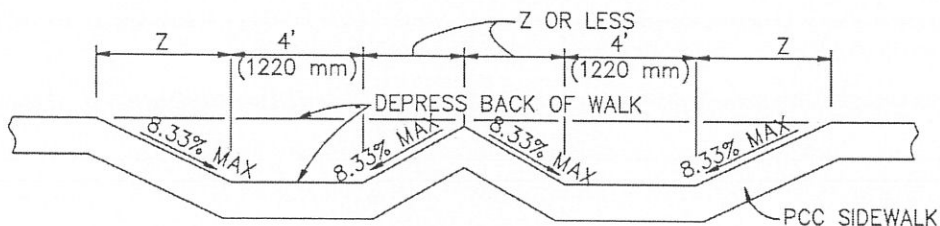
SECTION S-S
