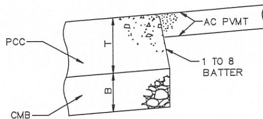
SECTION F-F
