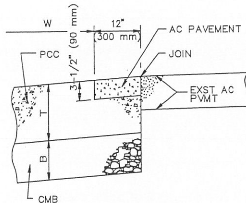
SECTION E-E
